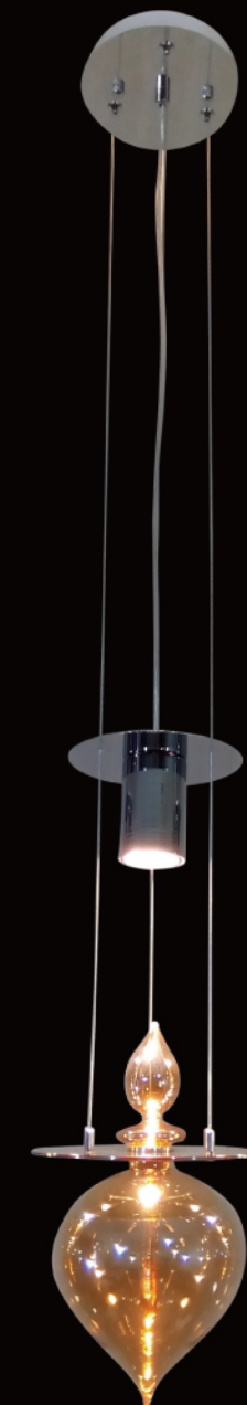
A8197-1 Vacuum Plating Glass GU10 1x5W 220V Ø140x180mm Amber
